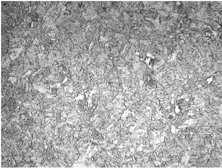
Figure 14. Appearance of the primary sorbitic structure after the 5000 h exposition of 100°C for 5000 h; except the sorbite the ferrite appears
