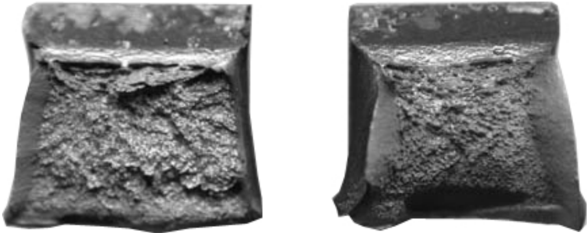
Figure 11. Fracture surface appearance of the steel 21MnTiB tempered at 200°C without the heat exposition at the test temperature (from left to right) -40°C and 20°C.
