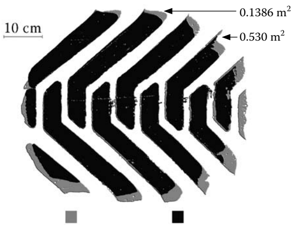
Figure 4. Contact patch of Alliance 600/55 R22.5 left tyre at Annaburger HTS 22.79 semitrailer rear axle
