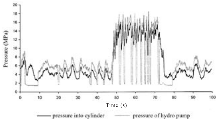
Fig. 7. Time dependent state of output pressure of hydraulic pump and of input pressure of hydraulic cylinder during ploughing with plough KUHN – draught control
