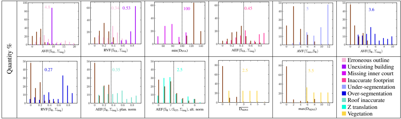
Figure 5: Error detection using one-against-all method (training set). ■: complement of each evaluated error. - -: computed threshold.
