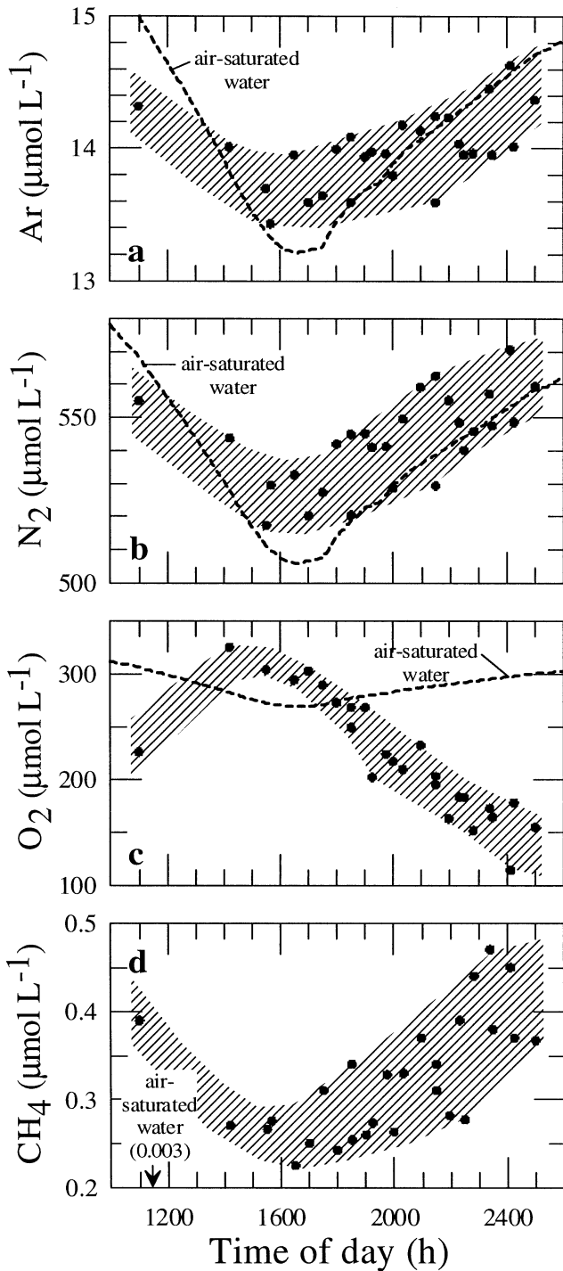
Fig. 6. Concentrations of Ar, N 2 , O 2 , and CH 4 in the stream. Dotted curves indicate atmospheric equilibrium concentrations calculated from the temperature record (Fig. 3). Shaded areas highlight trends inferred from the data.
