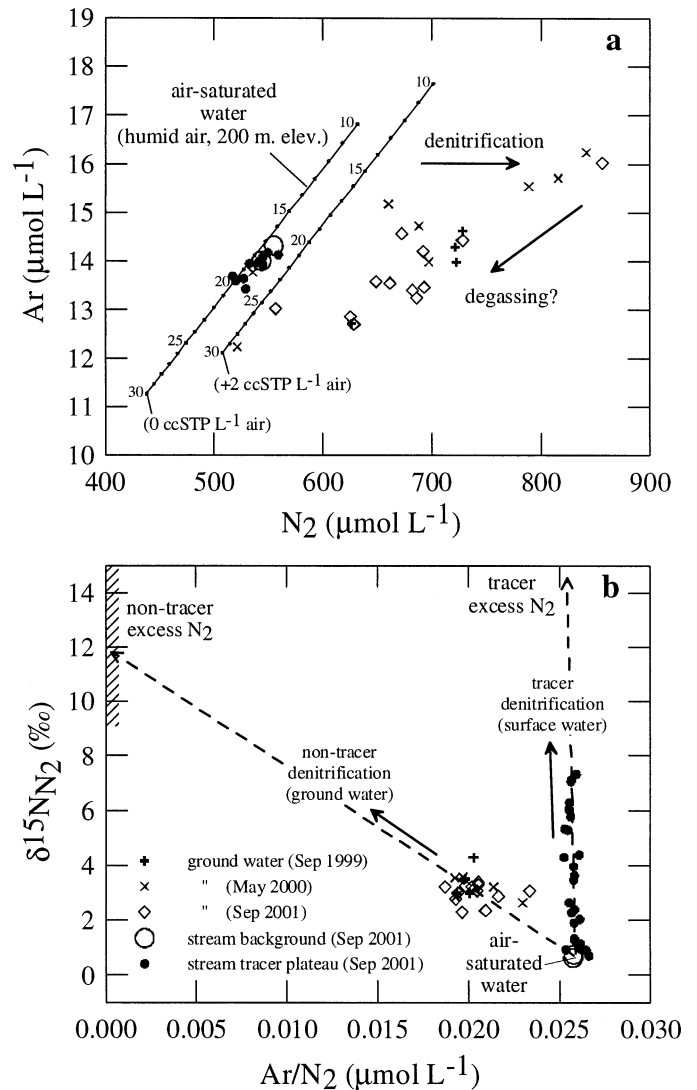
Fig. 7. Concentrations of Ar, N 2 , and δ 15 N[N 2 ] values in stream water and in groundwater from beneath the stream. (a) Curves indicate concentrations in equilibrium with air at 200 m elevation and 100% relative humidity, with 0 or 2 ccSTP L -1 of excess unfractionated air, at temperatures ranging from 10°C to 30°C. (b) Non-tracer groundwaters beneath the stream have large amounts of excess N 2 with only slightly elevated δ 15 N[N 2 ], whereas stream tracer plateau samples have small amounts of excess N 2 with much higher δ 15 N[N 2 ].
