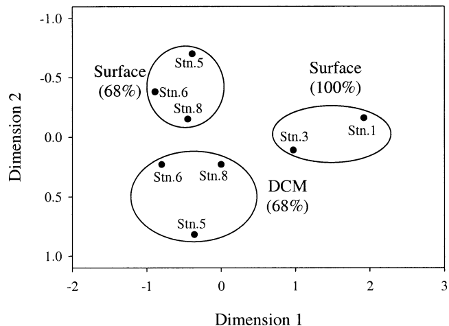
Fig. 2. Multidimensional scaling plot of the bacterial communities from North Pacific stations based on T-RFLP of 16S rRNA genes, which shows that samples from similar oceanographic settings were relatively similar to one another (circled clusters). The clusters were supported by UPGMA analysis, and the percentage of 100 bootstrap resamplings is indicated in parentheses. Like a tree-plot, which is essentially a one-dimensional visualization of a distance matrix, this plot is a two-dimensional visualization of the distance matrix. The coordinates for each sample in this plot are values that describe the samples' position within the overall community variation we observed on our transect. The stress of the plot is 0.045, which is well below the commonly held threshold of 0.15 for acceptability.
