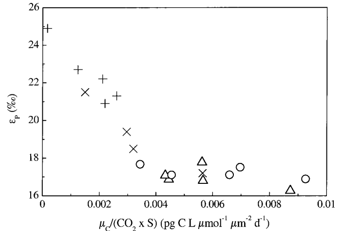
Fig. 6. Comparison of the relationship between \mu_c/(\text{CO}_2 \times S) and isotope fractionation ( \epsilon_p ) obtained by Bidigare et al. (1997) and in the present study. Chemostat data of the calcifying strain B92/11 ( \times ) and noncalcifying strain BT6 ( + ) incubated under continuous light at ca. 250 \mu\text{mol photons m}^{-2} \text{s}^{-1} . Symbols of the dilute batch culture as in Fig. 1.
