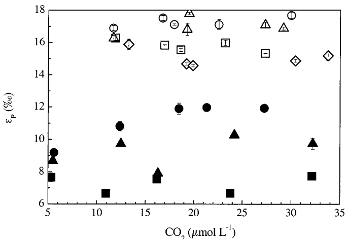
Fig. 2. Isotope fractionation ( \epsilon_p ) as a function of [\text{CO}_2] . Symbols and error bars as in Fig. 1.
