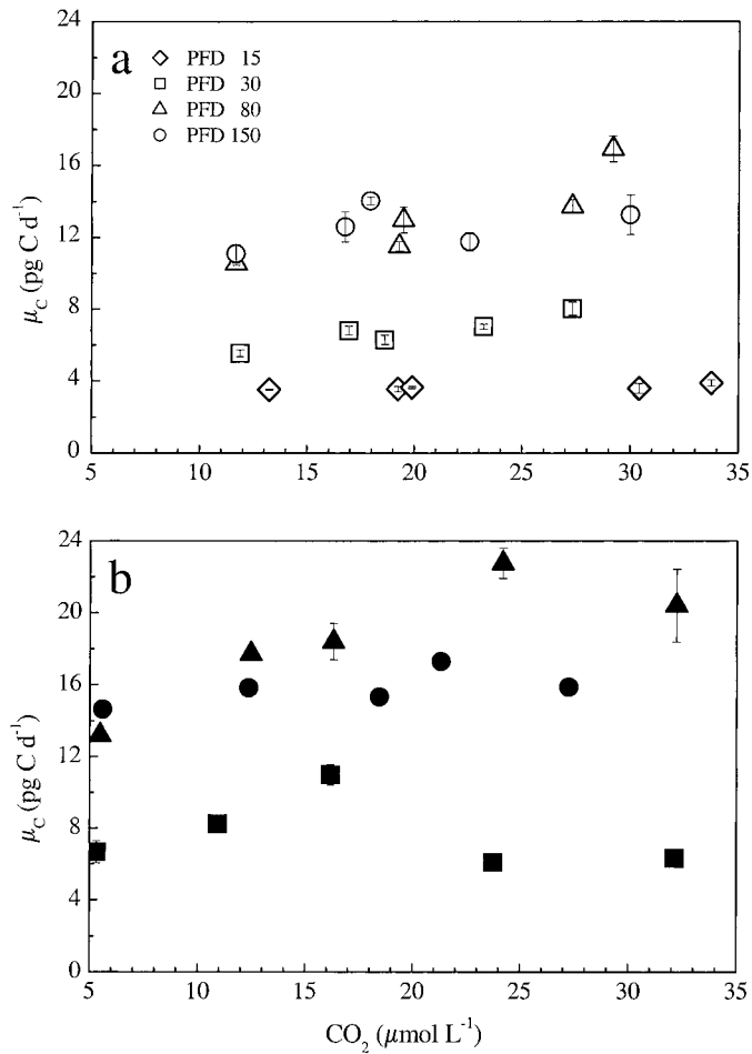
Fig. 1. Carbon-specific growth rates ( \mu_c ) as a function of [\text{CO}_2] at different light conditions. Open symbols and closed symbols represent the incubation at (a) continuous light and (b) the 16:8 h light:dark cycle. Symbols denote for light intensities PFD 15, PFD 30, PFD 80, and PFD 150. Error bars represent \pm 1 standard deviation of triplicate incubations ( n = 3 ).
