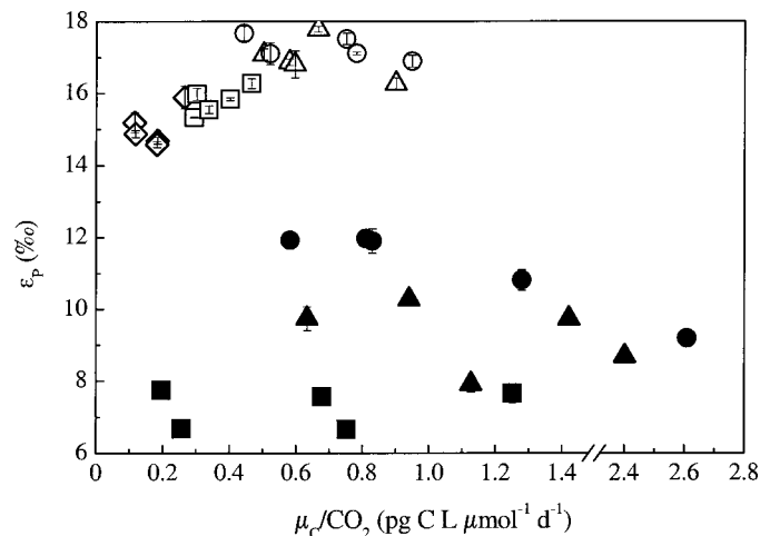
Fig. 4. Relationship between \mu_c/[\text{CO}_2] and isotope fractionation ( \epsilon_p ). Symbols and error bars as in Fig. 1.
