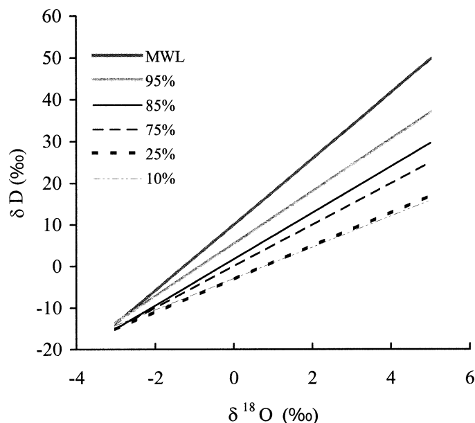
Fig. 6. Model data showing the behavior of \delta^{18}\text{O} and \delta\text{D} during evaporation (Gonfiantini 1986) from a initial composition similar to that shown in Fig. 6. With increasing relative humidity, the correlation between oxygen and hydrogen plots closer to the MWL.
