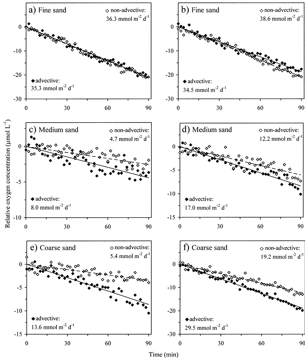
Fig. 5. Six examples of oxygen concentration time series at the (a, b) fine, (c, d) medium, and (e, f) coarse sand station. Oxygen concentrations are normalized to the same initial concentration and originate from the last 90 min of the advective (filled diamonds) and the first 90 min of the nonadvective stirrer setting (open diamonds). The trend lines represent linear regressions to oxygen depletion during the advective (solid line) and nonadvective stirrer setting (dashed line). The corresponding TOU values are indicated in the graphs.
