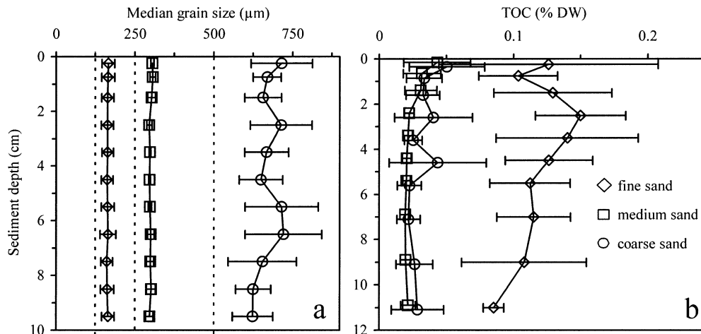
Fig. 3. (a) Median grain size, and (b) total organic carbon content (TOC) versus sediment depth. Marks represent the average (whiskers, SD) of three (grain size) and six replicates (TOC), respectively. Points are positioned in the center of the respective sediment layer. Depth intervals: 0–1 cm in 0.5-cm steps, 1–10 cm in 1-cm steps (grain size); 0–1 cm in 0.5-cm steps, 1–6 cm in 1-cm steps, 6–12 cm in 2-cm steps (TOC). Dotted lines in (a) represent the lower limits of the Udden-Wentworth size classes: fine, medium, and coarse sand (from left to right). In (b) points have been slightly shifted vertically to facilitate discrimination between the respective data series.
