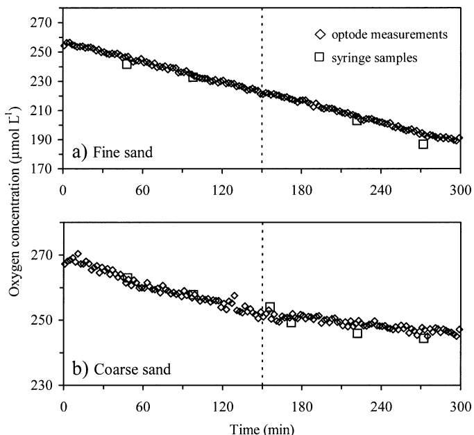
Fig. 4. Examples of oxygen depletion with time at (a) the fine, and (b) the coarse sand station. Diamonds represent the optode measurements, squares the oxygen concentrations of the syringe samples. The dotted lines at t = 150 min indicate the shift from the advective to the nonadvective stirrer setting.
