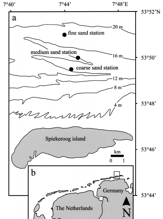
Fig. 1. (a) Location of the three stations and the bathymetry of the area (redrawn after Antia 1993). (b) The chain of West and East Frisian Islands. The box marks the area around the Island of Spiekeroog.
