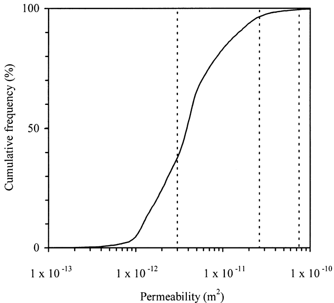
Fig. 9. Cumulative frequencies of the permeabilities of the German Bight according to the 1 \times 1 \text{ km}^2 grid (see legend of Fig. 8). Apart from minute errors that result from the simplifying equidistant cylindrical projection, the frequencies equal the proportion of the total seafloor area of Fig. 8 (approximately 29,000 \text{ km}^2 ) that is covered by sands of the respective permeabilities. The dashed vertical lines represent the permeabilities at the fine, medium, and coarse sand station (from left to right).
