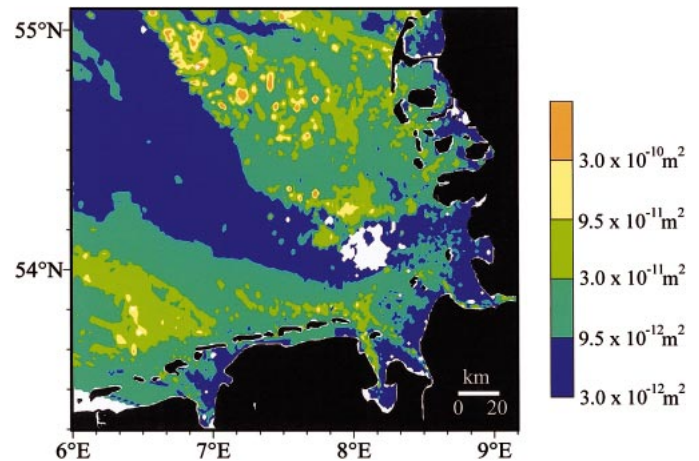
Fig. 8. Contour plot of the permeabilities of the German Bight as calculated based on grain size measures according to Krumbein and Monk (1943) using the median grain sizes and standard deviation in phi units. The standard deviation was inferred from the reported 25th and 75th percentile (data source: Marine Environmental Data Base, Federal Maritime and Hydrographic Agency of Germany). The permeabilities of the individual samples are transferred to an approximately 1 \times 1 \text{ km}^2 grid by triangulation with linear interpolation. Gridding and contour plotting were done with the software Surfer 6.01 (Golden Software Inc.). Blank parts in the plot mark areas that were not covered by samples (lower left corner) or where median grain sizes were below the sand size range (e.g., muddy area around 54^\circ\text{N} , 8^\circ\text{E} ).
