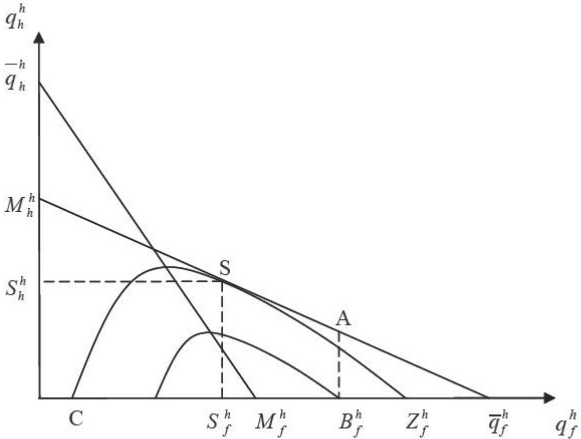
Figure 2: Reaction Functions
