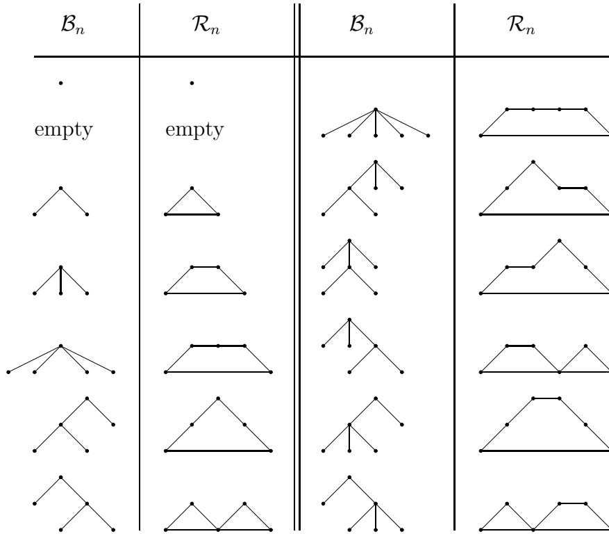
Figure 1: Short bushes and Riordan paths
