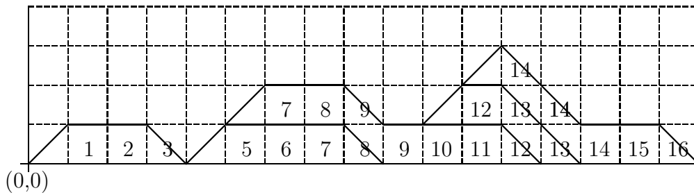
Figure 2: The (x + y) -labeling and strip decomposition
