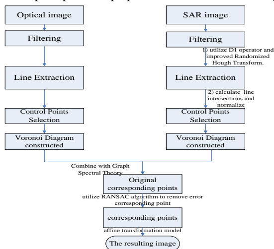
Fig. 1 Algorithm flowchart
