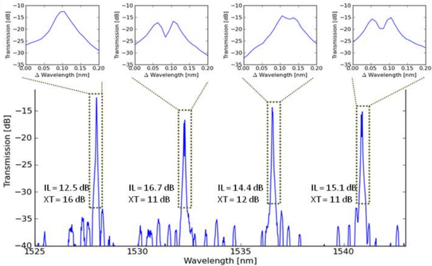
Figure 2: Transmissions spectrum taken at the drop port of an add-drop MRR (R = 20μm and gap 400nm) using TE-polarized light, illustrated with the insertion loss (IL) and crosstalk (XT), showing splitting of the resonances for some peaks and exhibiting unstable IL and XT.
