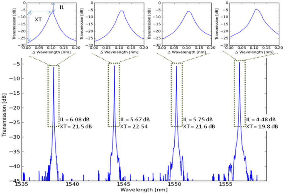
Figure 1: Transmissions spectrum taken at the drop port of an add-drop MRR (R = 20μm and gap 1μm) using TM-polarized light, illustrated with the nearly constant insertion loss (IL) and crosstalk (XT), showing the stable behavior of the subsequent resonances.
