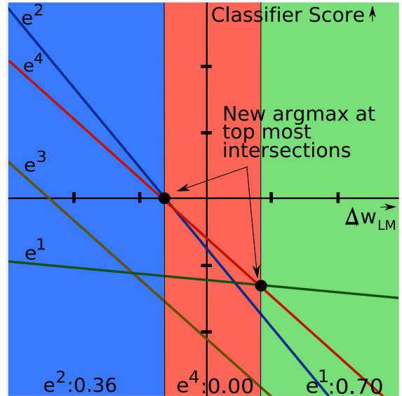
Figure 2: Illustration of how the model score assigned to each candidate translation varies during a line search along the coordinate direction w_{lm} with a starting point of (w_{lm}, w_{lm}) = (1.0, 0.5) . Each plotted line corresponds to the model score for one of the translation candidates. The vertical bands are labeled with the hypothesis that dominates in that region. The transitions between bands result from the dotted intersections between 1-best lines.
