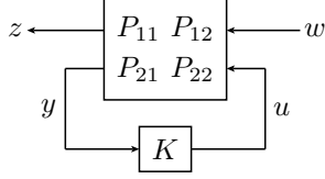
Figure 1: Closed-loop interconnection between a plant P and controller K
