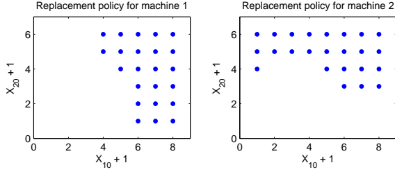
Figure 1: Centralized replacement policy at t = 0 .
