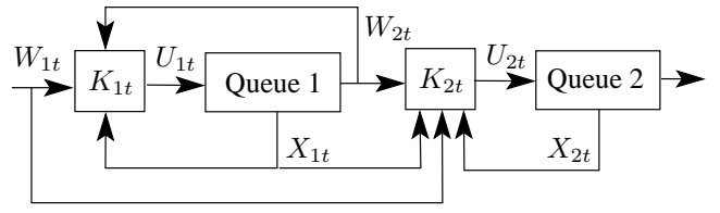
Figure 3: Admission control for two queues in series
