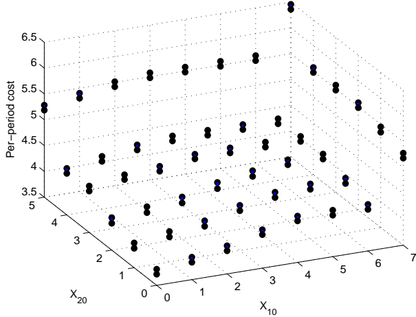
Figure 2: Performance gap between centralized and decentralized replacement policies.
