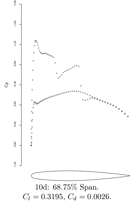
Figure 10: Onera M6 Wing. Mach 0.840, Angle of Attack 3.06^\circ , 192 \times 32 \times 48 Mesh. C_L = 0.3041 , C_D = 0.0131 . H-CUSP scheme.
