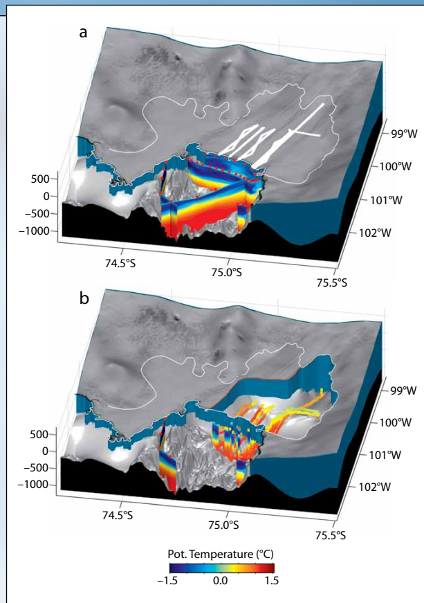
Figure 3. (a) Perspective view of Pine Island Bay showing surface and seabed topography along with potential temperature sections measured from the Palmer in January 2009. Bold white lines on the surface of Pine Island Glacier indicate the geographic location of Autosub3 tracks beneath the floating ice shelf, whose boundaries are indicated by the faint white line. The fast-flowing central part of the ice shelf is apparent from the dark, linear, surface features apparent in the Moderate Resolution Imaging Spectroradiometer (MODIS) imagery that is draped over the surface topography. (b) As in (a), but with most of the ice shelf cut away to reveal potential temperature measured along Autosub3 tracks.
