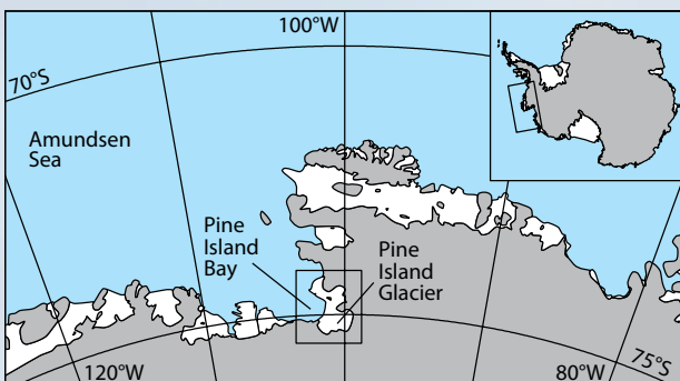
Figure 1. Map of Antarctica (inset) and enlargement of the eastern Amundsen Sea coastline showing grounded ice (grey) and floating ice shelves (white). The box outlining Pine Island Bay indicates the area shown in Figure 3.
