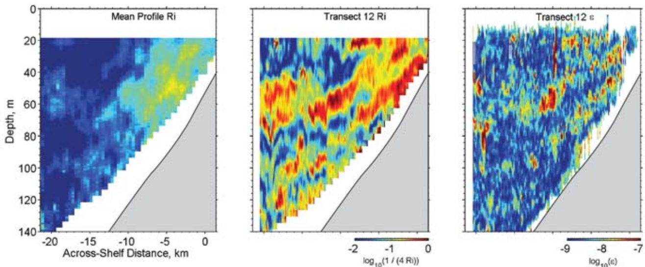
Figure 7. Thermal wind Richardson number ( Ri ) compared to observed Ri and \epsilon , each computed from data corresponding to the cross-shelf transect marked +197 h in Figure 2. The left panel shows inverse Ri computed using thermal wind shear alone, the middle panel inverse Ri computed from the observed shear (4-m scale) and the right panel the observed \epsilon . The critical component of the observed shear is that due to internal waves. Clearly, the thermal wind shear does not display the structure that is observed in the turbulence, \epsilon . Adapted from Avicola et al., 2007
