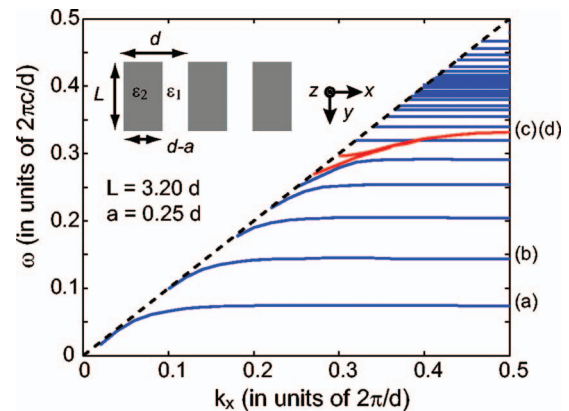
FIG. 1. (Color) Guided-mode band diagram for TM polarization (first Brillouin zone) when L=256 nm, d=80 nm, a=20 nm. Shown are two degenerate surface modes (red curves) and a series of effective dielectric slab modes (blue curves). The dashed line is the light line in vacuum. Inset shows the schematic of a metallic film with periodic slits: a is the slit width, d is the periodicity, and L is the film thickness. The gray regions indicate metal ( \epsilon_2 ) and the white regions represent vacuum ( \epsilon_1=1 ).
