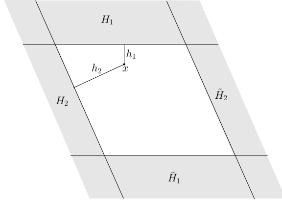
Figure 4: Diagram for the Proof of Lemma 5.4.
