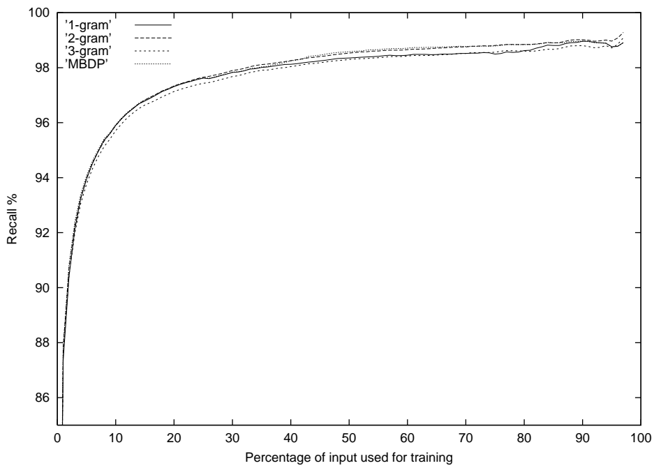
Figure 8 Improvement in recall with training size.
