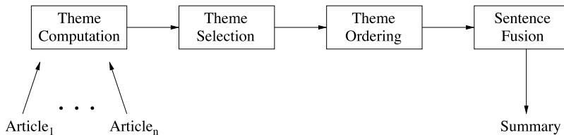
Figure 2 MultiGen architecture.
