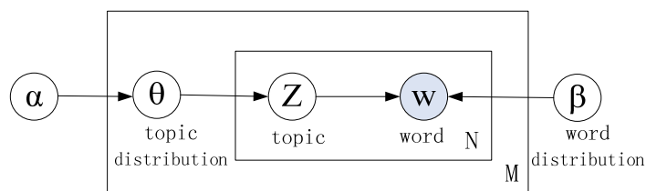
Fig. 2 The original LDA
