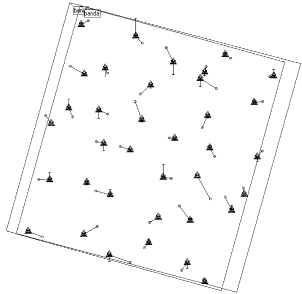
Figure 3. The errors of RPC model with bias-and-drift refinement applied (all the points are GCPs).
