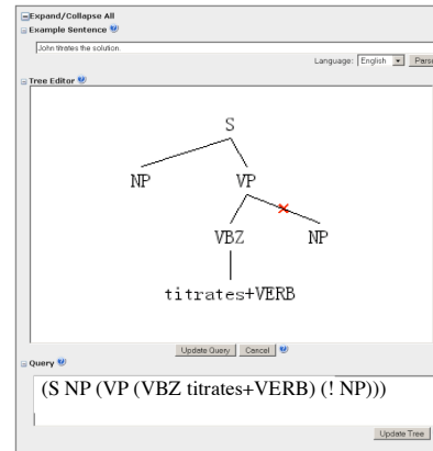
Figure 2. Resulting query
