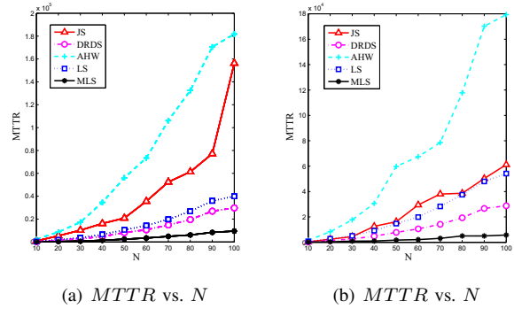
Fig. 9. MTTR comparison when N increases from 10 to 100. M = 100 , (a) \theta_A = \theta_B = 0.5, n_G = 1 ; (b) \theta_A = \theta_B = 0.3, n_G = 1
