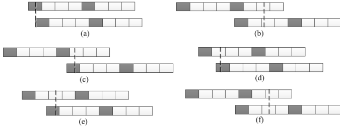
Fig. 4. Illustrations of Theorem 1's proof
