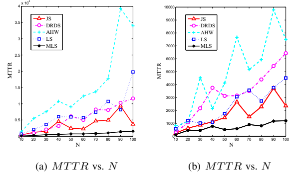
Fig. 11. MTTR comparison for asymmetric users. N \in [10, 100] , M = 100 , (a) \theta_A = 0.5, \theta_B = 0.2, \theta_G = 0.1 ; (b) \theta_A = 0.5, \theta_B = 0.8
