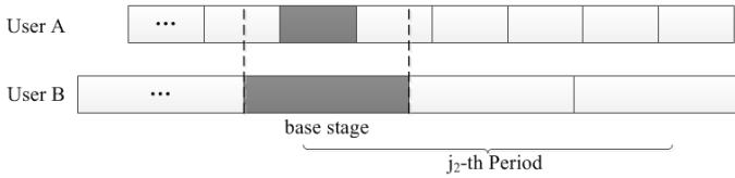
Fig. 5. Example of Lemma 5.2 when p_B \geq 2p_A
