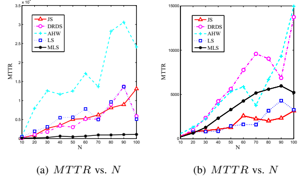
Fig. 10. MTTR comparison for asymmetric users when N increases from 10 to 100. M = 100 , (a) \theta_A = \theta_B = 0.2, \theta_G = 0.1 ; (b) \theta_A = \theta_B = 0.8
