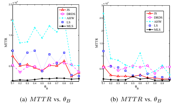
Fig. 12. MTTR comparison for asymmetric users when \theta_B increases from 0.1 to 1. M = 100, N = 50 , (a) \theta_A = 0.2 ; (b) \theta_A = 0.5
