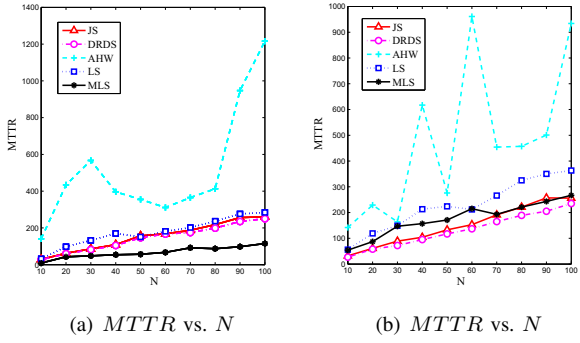
Fig. 8. MTTR comparison for symmetric users when N increases from 10 to 100. M = 100 , (a) \theta_A = \theta_B = 0.2 ; (b) \theta_A = \theta_B = 0.8
