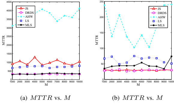
Fig. 7. MTTR comparison as M increases from 1000 to 10000 when N = 10, n_A = 5, n_B = 5 : (a) n_G = 1 ; (b) C_A = C_B .
