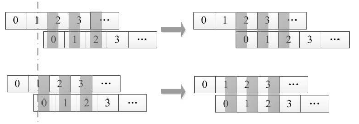
Fig. 1. Transform non-aligned slots to aligned ones
