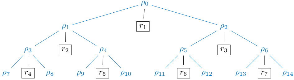
Figure 2: A binary tree within the lookup tree
