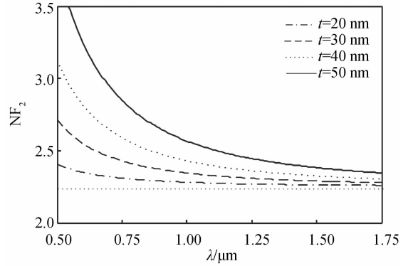
Fig. 6 Noise factor variation of periodic stripe LRSPPs with different t
