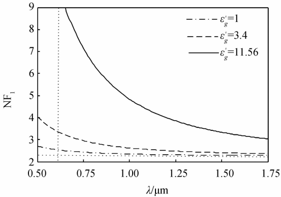
(a) Noise factor of SPPs with different gain mediums
