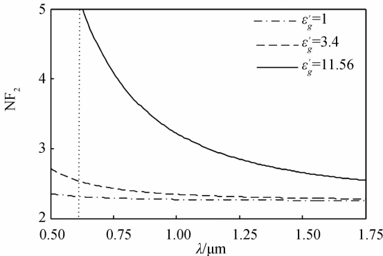
(b) Noise factor of periodic stripe LRSPPs with different gain mediums
