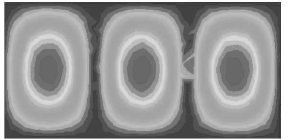
Fig. 3 Electromagnetic field distribution of LRSPPs with a thin metal film
