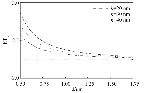
Fig. 7 Noise factor variation of periodic stripe LRSPPs with different h
