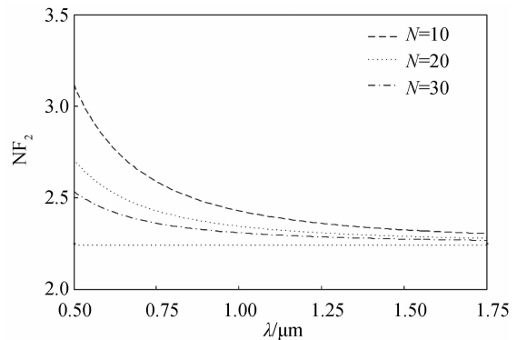
Fig. 8 The noise factor variation of periodic stripe LRSPPs with different N
