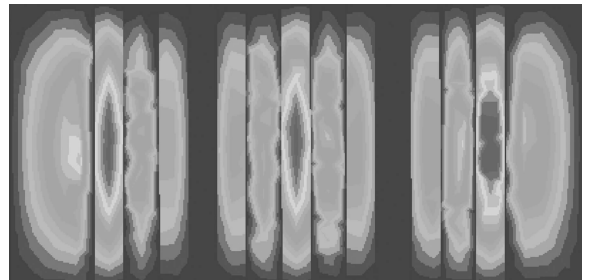
Fig. 4 Electromagnetic field distribution of periodic stripe LRSPPs
