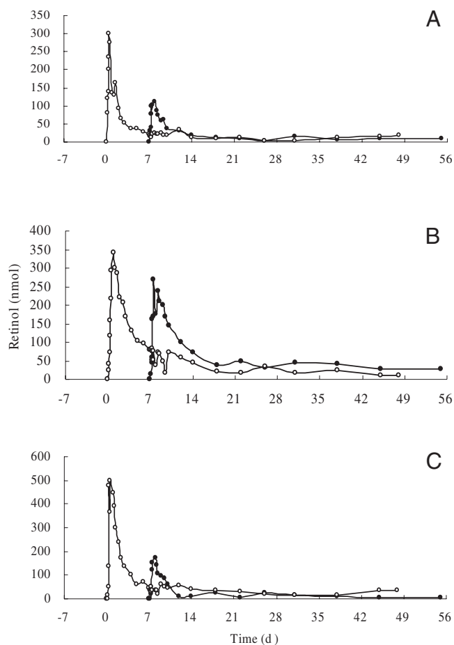
FIGURE 3. Serum response curves of [^{13}\text{C}_{10}] retinol from retinyl acetate (○) and [^2\text{H}_5] retinol from spirulina \beta -carotene (●) in 3 subjects. A, subject 1; B, subject 6; C, subject 7.
