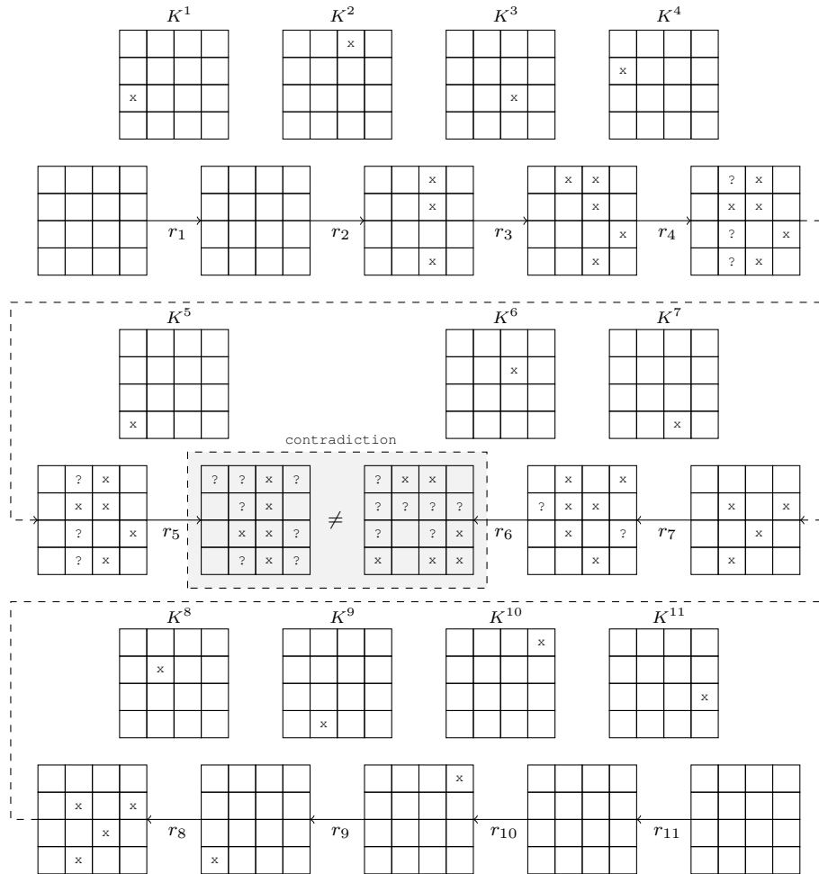
Fig. 3: Related-Key Impossible Differential Trail for 11 round SKINNY 64/128
