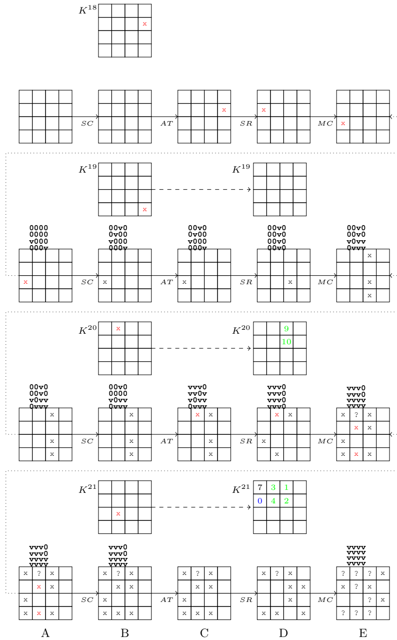
Fig. 5: Trail for the backward 4 rounds (the values of active nibbles in red are functions of \delta_1, \delta_2 )
