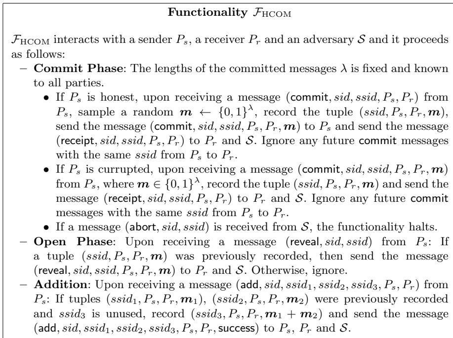
Fig. 1. Functionality \mathcal{F}_{\text{HCOM}}
