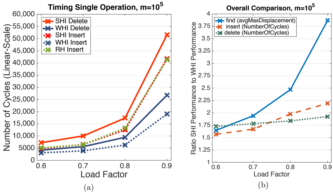
Figure 4: Comparison of the performance of methods insert and delete in Robin Hood (where ties-break with FCFS), SHI [7] and WHI (our scheme). Plot (a) summarizes the results from experiments conducted 10^3 times on a table of size m = 10^5 with varying load factors. In each experiment, we measured the number of CPU cycles executed by a single call of method insert or delete. Plot (b) depicts the ratio between the performance of SHI to WHI.
