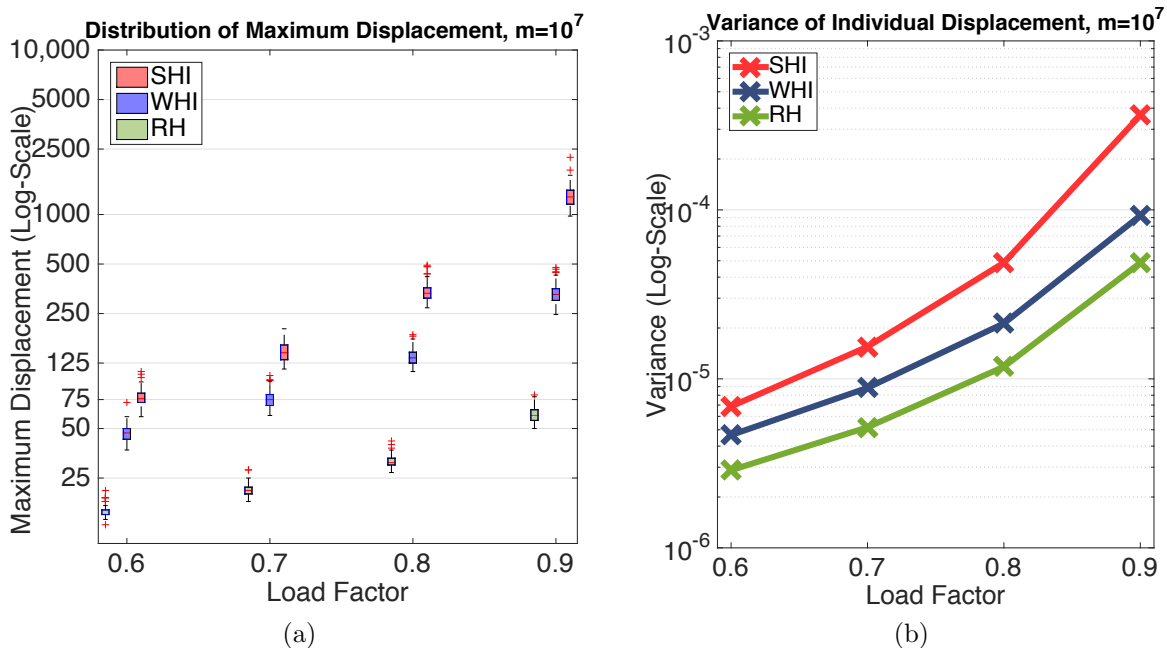
Figure 3: Comparison of the displacement of items in Robin Hood (where ties-break with FCFS), SHI [7] and WHI (our scheme). The plot summarize results from experiments run 100 times on a table of size m = 10^7 with varying load factors: (a) maximum displacement; (b) variance of individual displacement.
