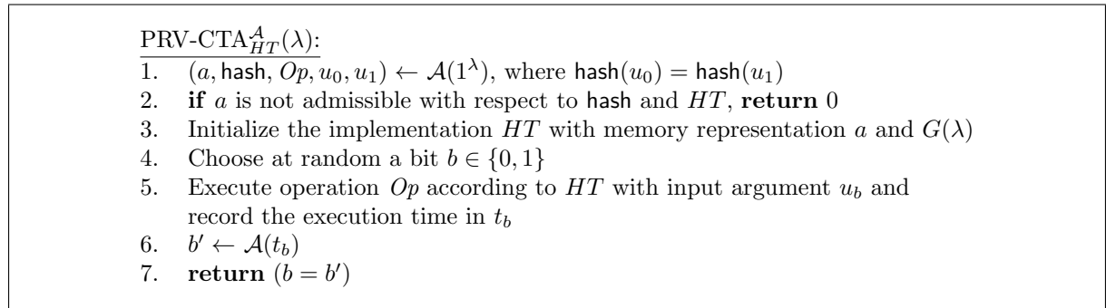
Figure 1: Indistinguishability game for the security of a hash table against collision-timing attacks.
