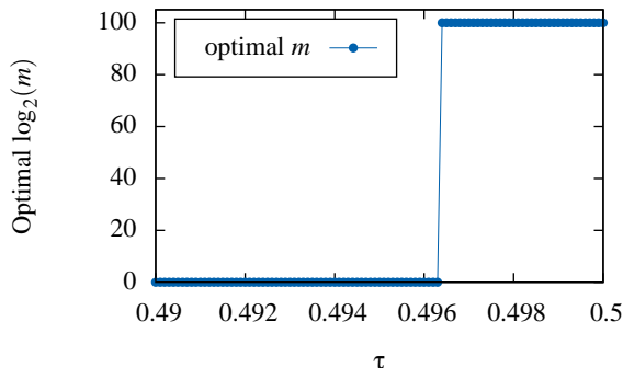
Fig. 1: The change of optimal m for solving \text{LPN}_{100, \tau}
