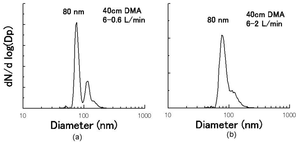
Fig. 3. The size distribution of a DMA outlet aerosol (incense smoke) measured by SMPS (TSI model 3071 with model 3010). The aerosol flow rate of the DMA was changed from 0.6 to 2 L/min.
