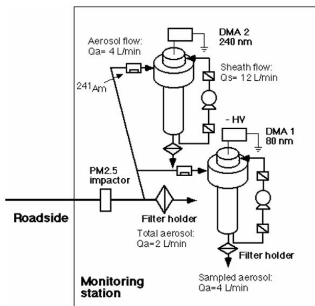
Fig. 1. The sampling train at the road-side at Ikegami-shincho.
