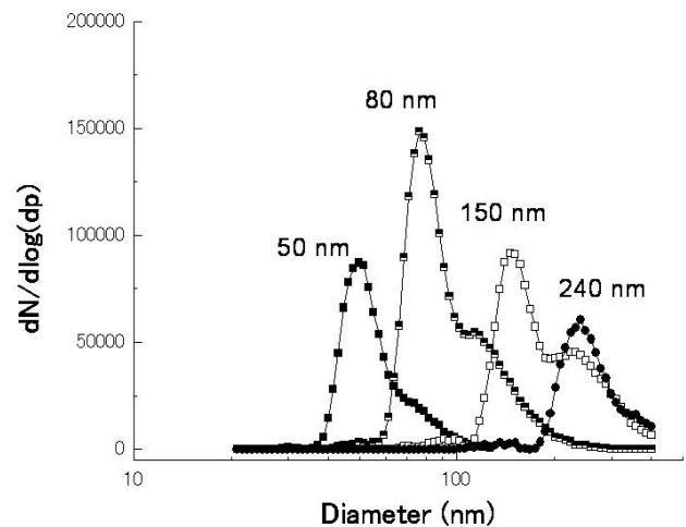
Fig. 4. The size distribution of a DMA outlet aerosol (incense smoke) measured by SMPS (TSI model 3071 with model 3010). The sheath flow rate was set at 12 L/min and the aerosol flow rate at 4 L/min.
