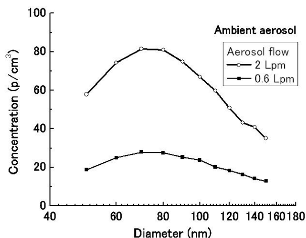
Fig. 2. The particle concentration of an ambient (indoor air) aerosol, measured at the DMA outlet using a condensation particle counter (TSI model 3022).
