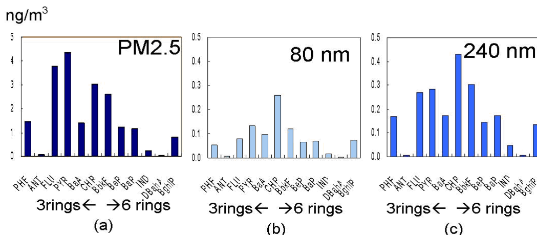
Fig. 7. PAH concentrations in samples collected at Ikegami-shincho.
