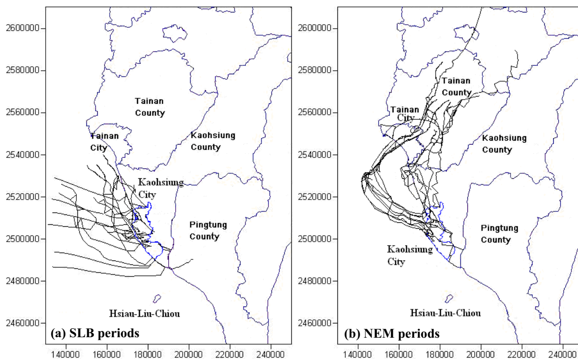
Fig. 6. Backward trajectories of air parcel transported toward the inland sites in the coastal region of southern Taiwan during (a) SLBs and (b) NEM periods (x- and y-axis legends are UTM in meter).
