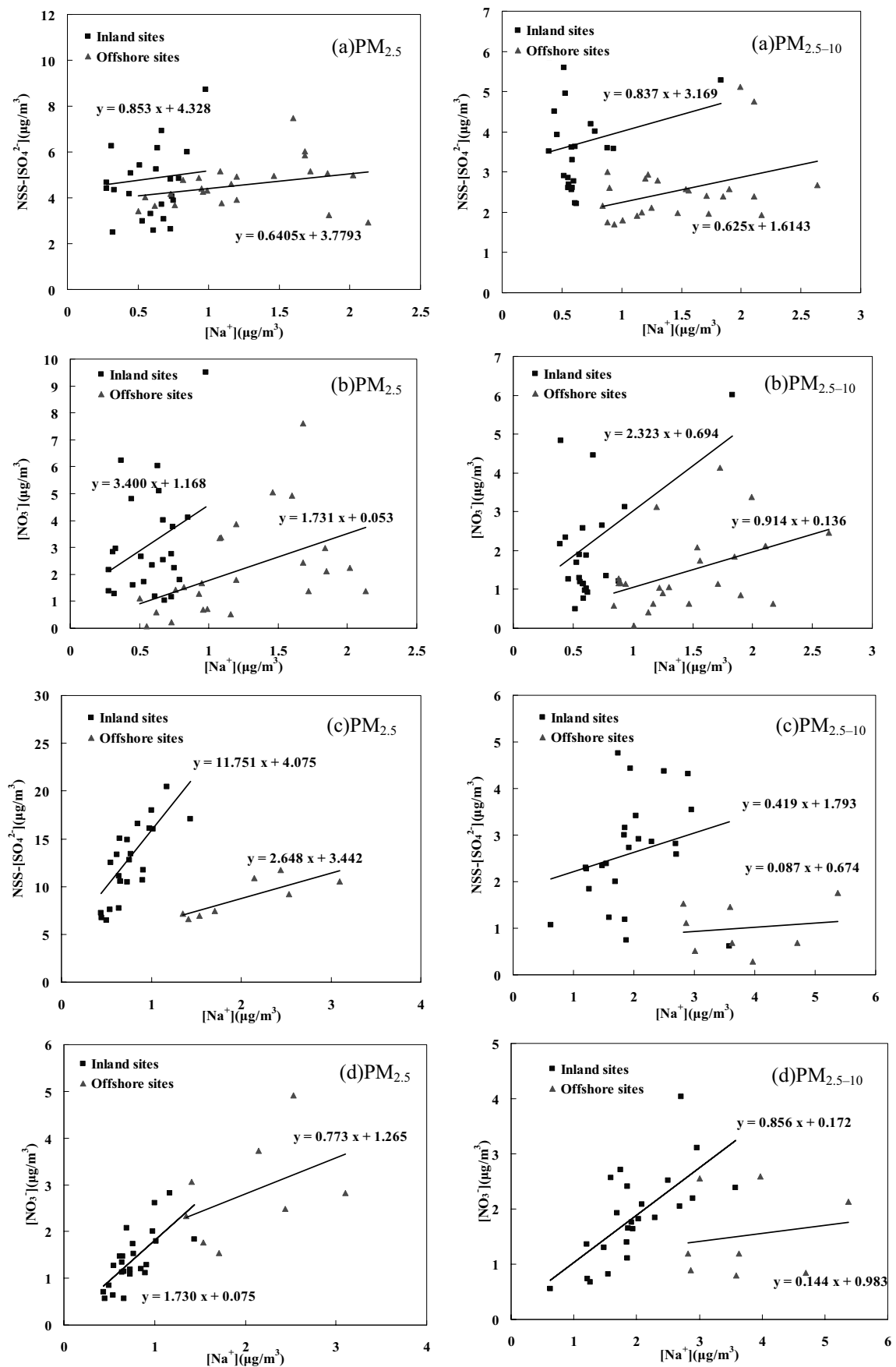
Fig. 7. \text{nss-}[\text{SO}_4^{2-}] to [\text{Na}^+] and [\text{NO}_3^-] to [\text{Na}^+] ratios for \text{PM}_{2.5} and \text{PM}_{2.5-10} during (a) (b) SLBs and (c) (d) NEM periods.
