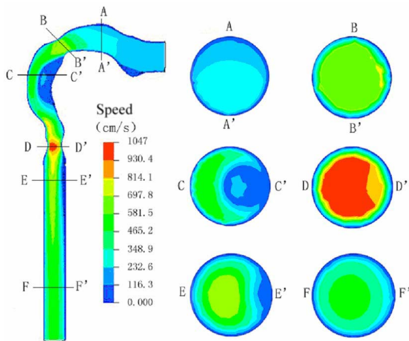
Fig. 4. Velocity profiles in the oral airway for Q_{in} = 30 \text{ l/min} . The left panel exhibits mid-plane ( Y = 0 plane) velocity contours. The right panels are the different cross-sectional views.
