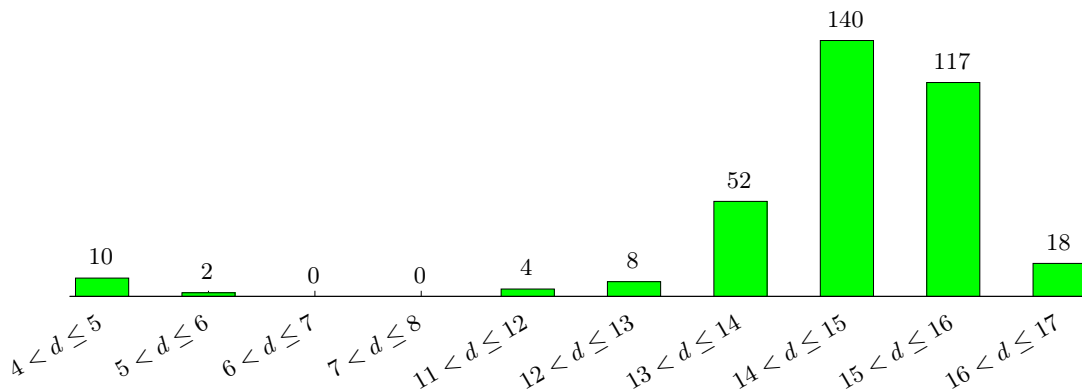
Fig. 3 – Log of the lowest indices of colliding tweak polynomials for every \mathbb{F}_{2^{32}} representations using the 351 degree 32 irreducible pentanomials over \mathbb{F}_2 .
