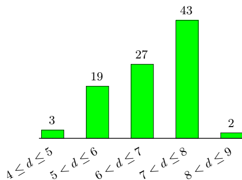
Fig. 2 – Log of the lowest indices of colliding tweak polynomials for every \mathbb{F}_{2^{16}} representations using the 94 degree 16 irreducible pentanomials over \mathbb{F}_2 .
