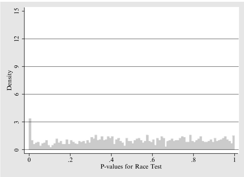
Figure 2 Distribution of p-values for race chi-squared tests
