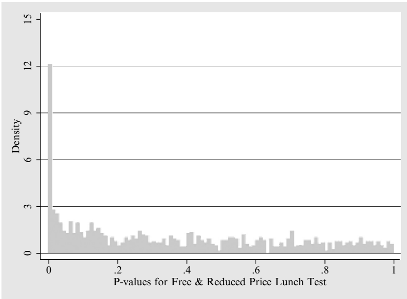
Figure 3 Distribution of p-values for subsidized lunch chi-square tests
