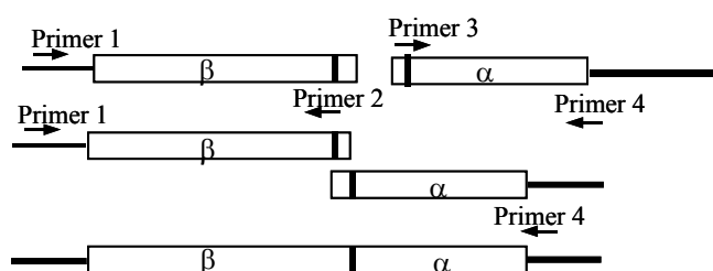
Figure 1. Construction of tethered-bLH and -bFSH by overlapping PCR mutagenesis.
