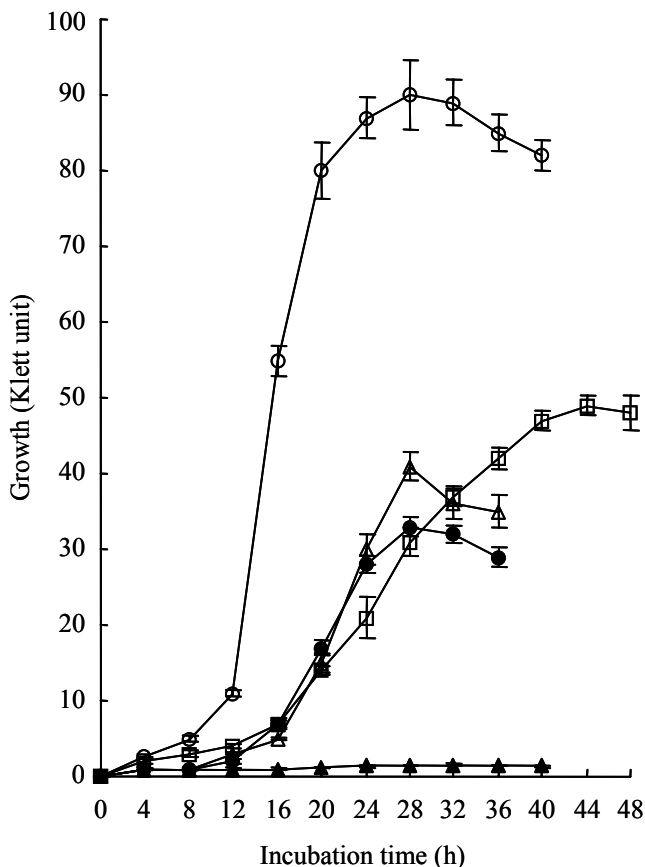
Figure 1. Growth of strain 9RCC5 in a basal medium together with the medium minus certain ingredients. Basal medium (○), minus casein hydrolysate (□), minus VFA (Δ), minus hemin (●), and minus vitamins (▲).
