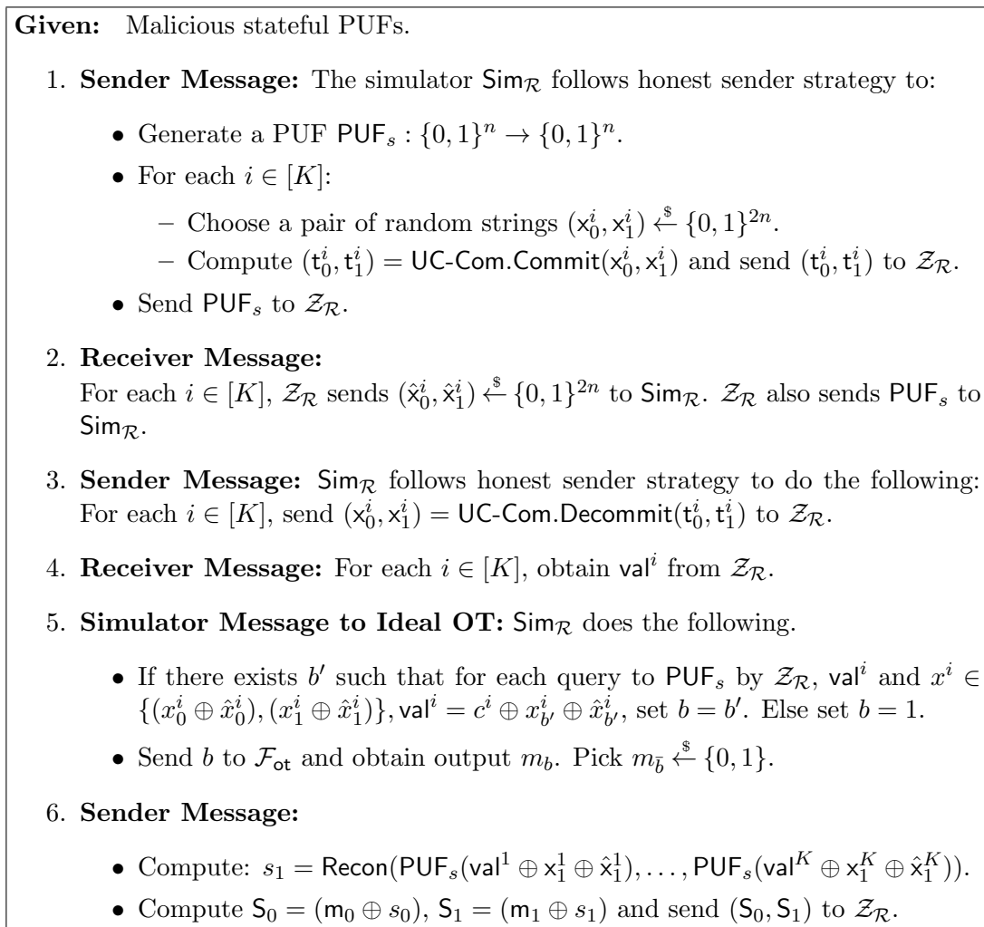
Figure 23: Receiver Simulation for K OTs (with \leq \ell leakage).
