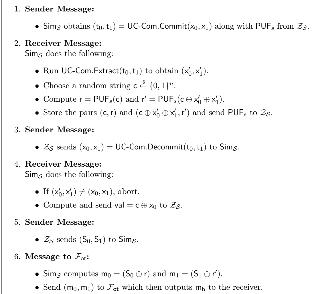
Figure 11: Simulation strategy against a malicious sender.
