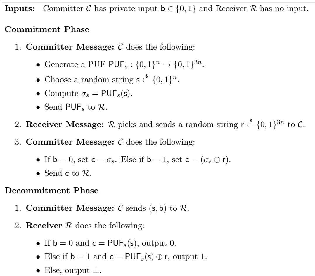
Figure 19: Protocol for Ideal Commitment in the malicious stateless PUF model with encapsulation.
