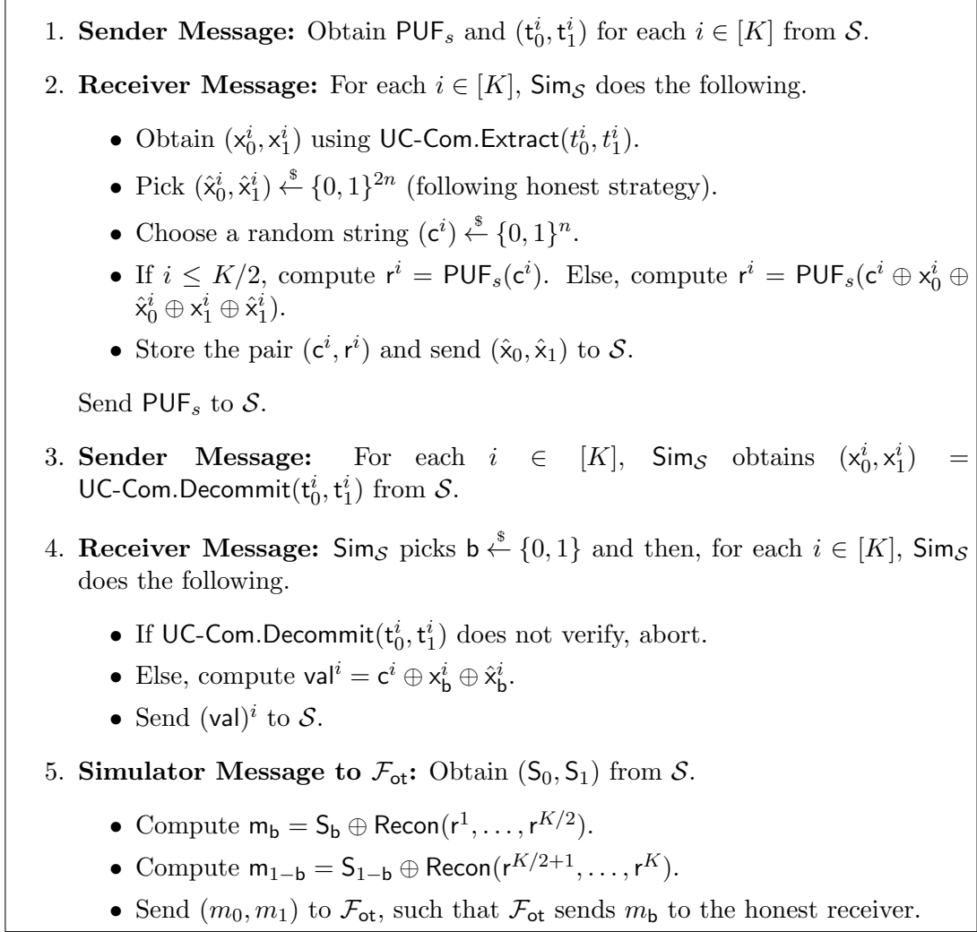
Figure 22: Sender simulation for K 2-choose-1 OTs (with at most \ell leakage) in the malicious stateful PUF model.
