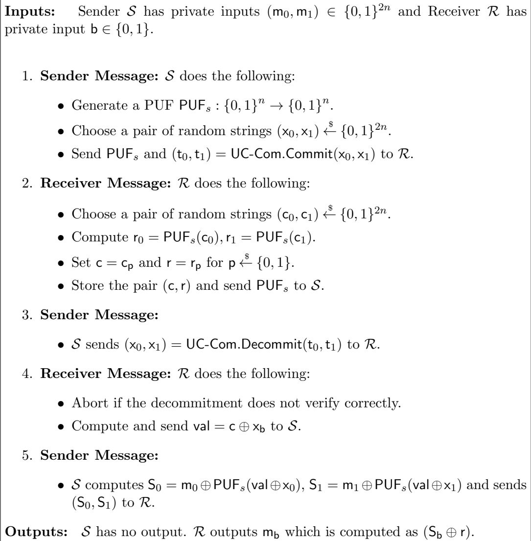
Figure 1: Protocol \Pi^1 for 2-choose-1 OT in the malicious stateless PUF model.
