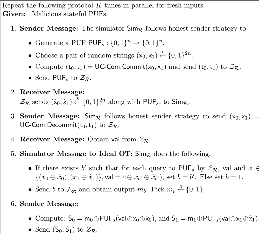
Figure 14: Receiver Simulation for K OTs (with \leq \ell leakage).
