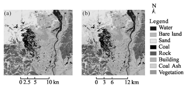
Fig.5 (a) Land cover produced by sole decision tree and (b) land cover produced by multi-subregions decision tree
