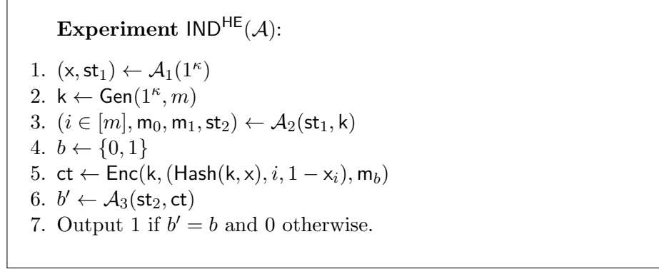
Fig. 6: The \text{IND}^{\text{HE}}(\mathcal{A}) Experiment
