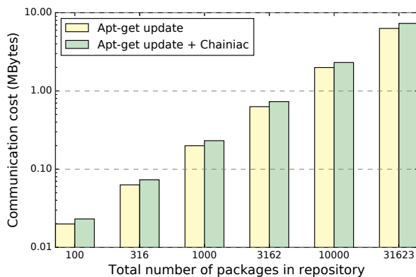
Figure 9: Communication cost to get new repository state
