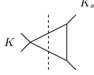
Figure 2: Double-cut of a Triangle
