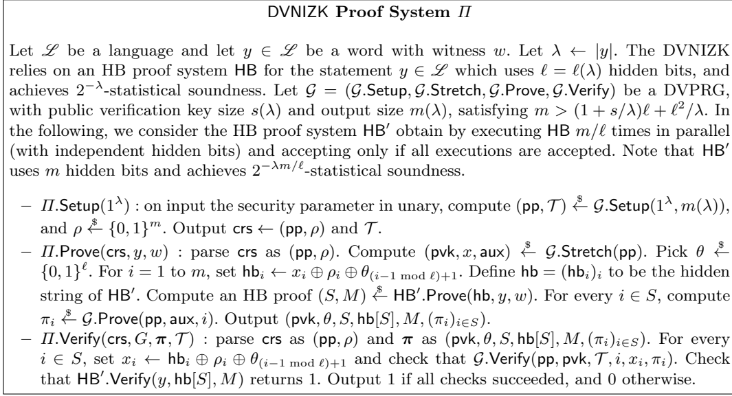
Fig. 2. Designated-verifier non-interactive zero-knowledge proof system \Pi for a language \mathcal{L} using a DVPRG \mathcal{G} and an HB proof system HB
