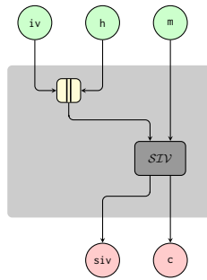
Figure 4: DAE-N/MRAE secure scheme from SIV mode.
