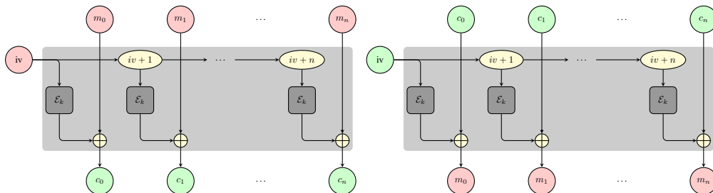
Figure 1: Example on key extraction using CTR-mode. By supplying the same IV twice, the attacker can wrap a key and then encrypt the resulting wrapping, again using the same IV. This leads to the leakage of the key.
